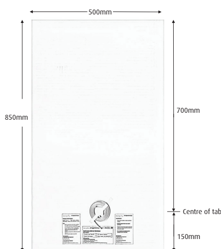
Demister 70W 500w x 850h mm TMD 70
