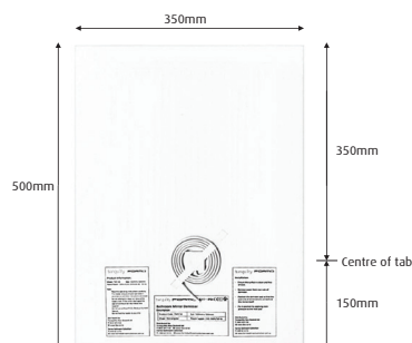
Demister 30W 350w x 500h mm TMD 30
