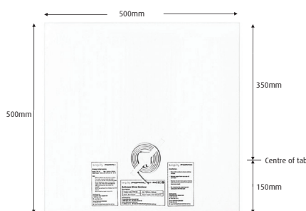
Demister 50W 500w x 500h mm TMD 50
