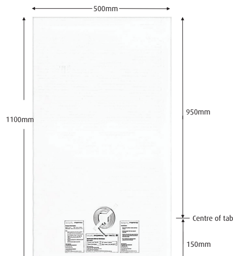
Demister 90W 500w x 1100h mm TMD 90
