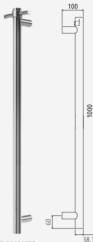
POLISHED PRV1000
