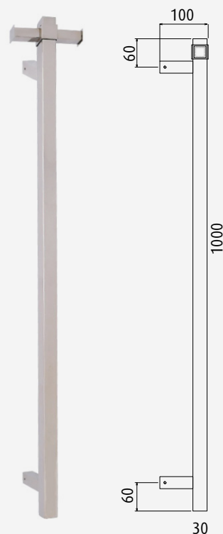
POLISHED PSV1000
