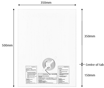
Demister 30W 350w x 500h mm TMD 30
